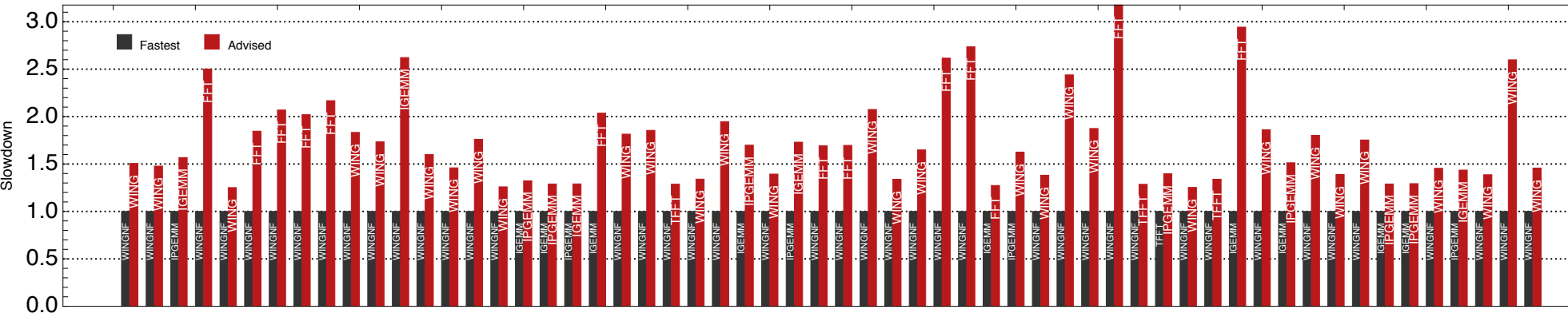
CUDNN v7.5.0.56 Heuristic Discrepancy (BatchSize = 32)
