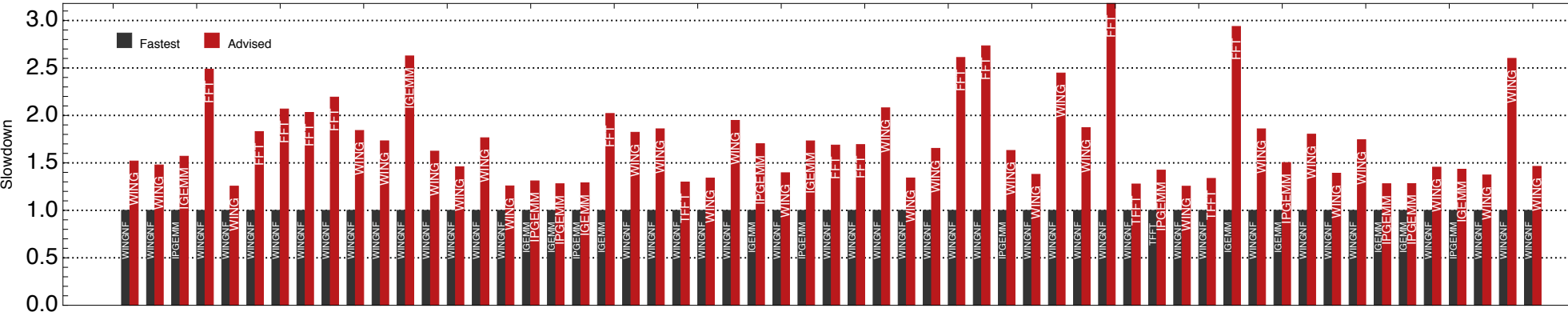
CUDNN v7.5.1.10 Heuristic Discrepancy (BatchSize = 32)
