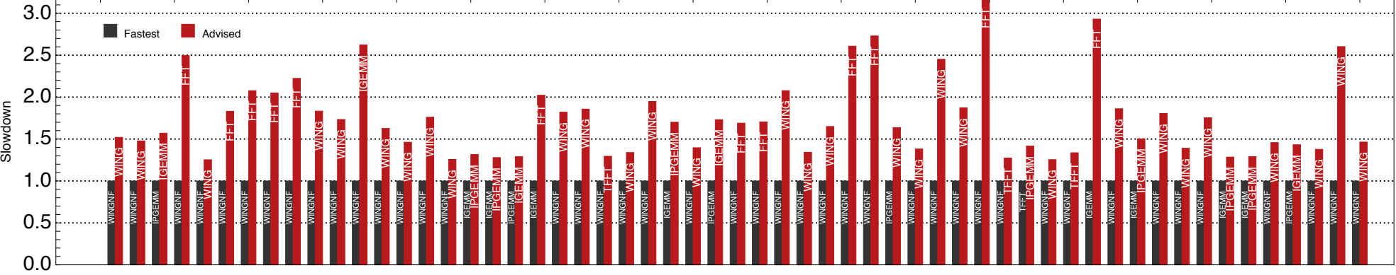
CUDNN v7.6.0.64 Heuristic Discrepancy (BatchSize = 32)
