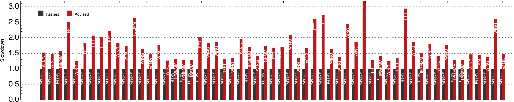
CUDNN v7.6.2.24 Heuristic Discrepancy (BatchSize = 32)
